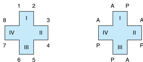
Figure 32-2. Uroporphyrin III. A (acetate) = —CH 2 COOH; P (propionate) = —CH 2 CH 2 COOH.
