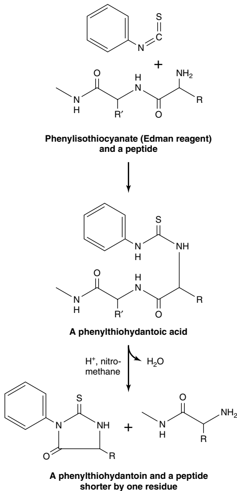
Figure 4-6. The Edman reaction. Phenylisothiocyanate derivatizes the amino-terminal residue of a peptide as a phenylthiohydantoin acid. Treatment with acid in a nonhydroxylic solvent releases a phenylthiohydantoin, which is subsequently identified by its chromatographic mobility, and a peptide one residue shorter. The process is then repeated.
